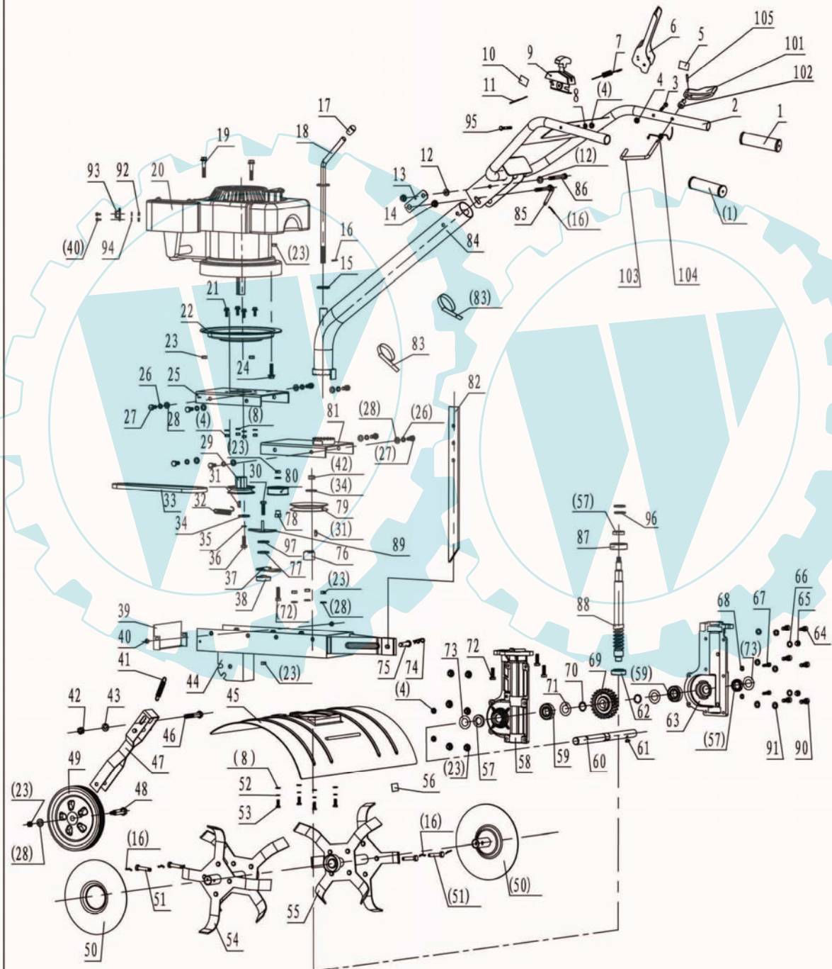
BOM OF TDS60A(Old model:TL60A1)
